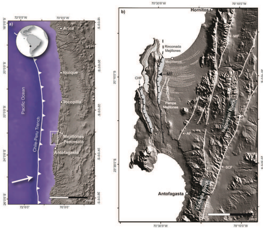
Figure 1. a) Shaded relief map of northern Chile made from SRTM 90 data. The Mejillones Peninsula is bordered by a white rectangle. The white arrow represents the convergence at 65 mm/ y and oriented \sim 75^{\circ}\text{E} [Angermann et al., 1999]. b) Shaded relief map of the Mejillones Peninsula elaborated by using SRTM 90 data. 1 and 2 indicate the Mejillones and Jorgino horst, respectively. Dotted polygons represent uplifted marine terraces of Middle-Late Pleistocene age. White segmented lines in Pampa Mejillones are paleo-beach ridges. Black lines in the Mejillones Peninsula and white lines further east are normal faults in the locality. The Mejillones Fault scarp is represented by small tick marks. Yellow circles (A and B) correspond to the sites where we measured the altitude in order to estimate the thickness of the alluvial deposits in the Pampa Mejillones.
