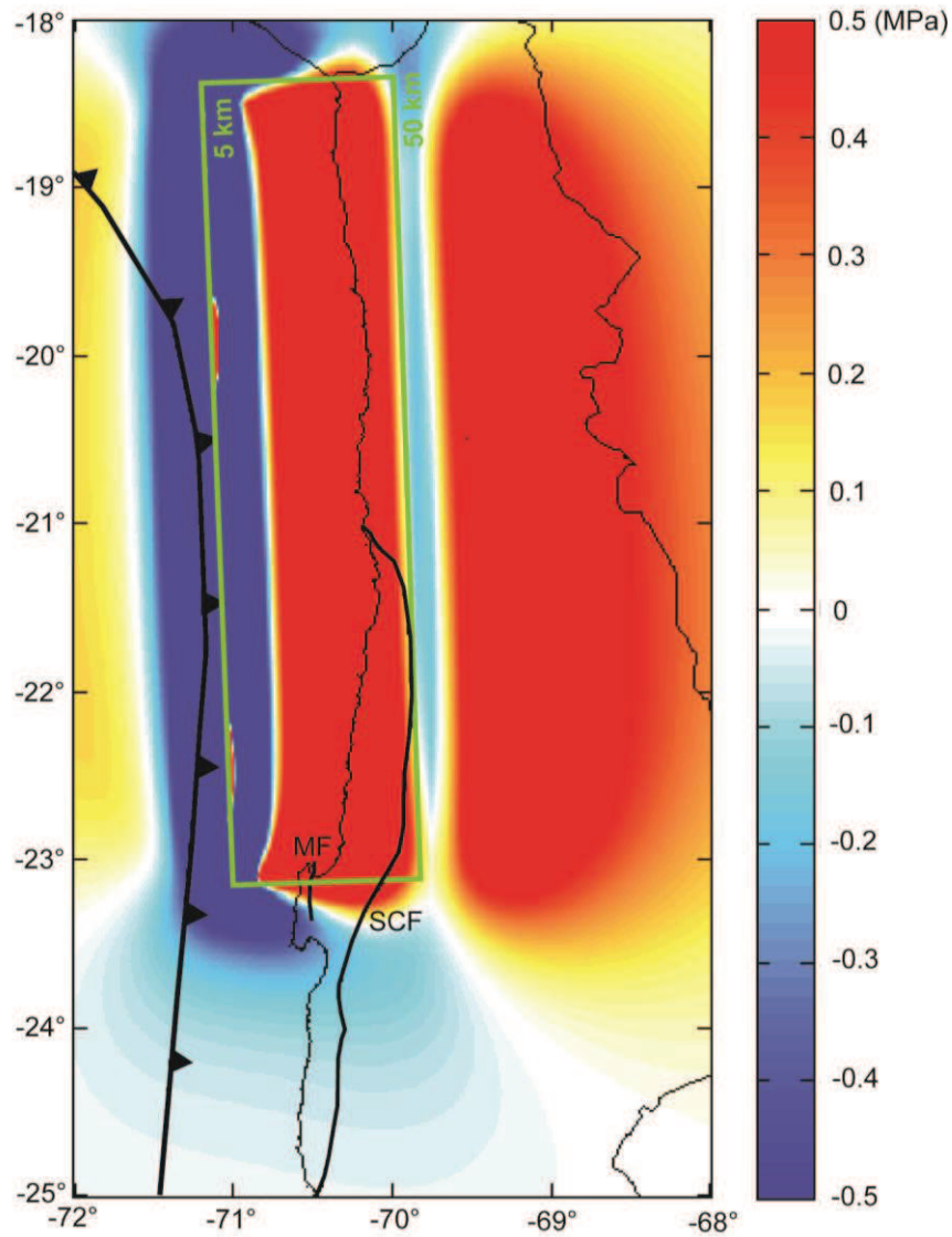
Figure 3. Model 1. Superficial (0 km depth) coseismic CSC model for the Iquique 1877 Earthquake. This model considers 8.66 m of coseismic slip homogeneously distributed along a rupture oriented N5°W/20°E, coupled between 5 and 50 km depth, and compatible with a M_w \sim 8.8 . Red zones correspond to positive CSC where tension is favoured. Blue areas are zone where the CSC is negative and thus tension is disadvantaged. The black dented line is the trench. Black lines are the Mejillones (MF) and Salar del Carmen (SCF) faults. Green rectangle simulates the seismogenic zone.
