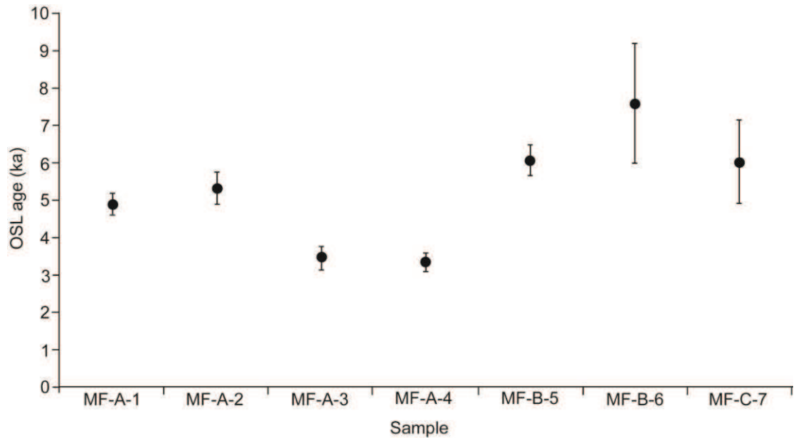
Figure 15. Plot showing the OSL ages ( 1\sigma uncertainties) obtained from trenches dug along the Mejillones Fault.
