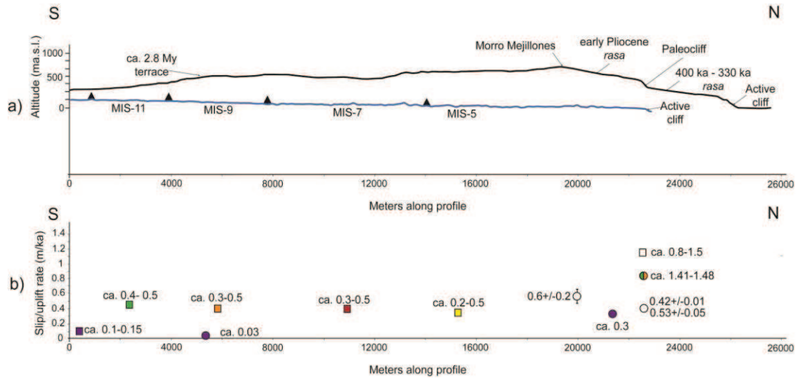
Figure 10. a) NS Topographic profiles of the Morro Mejillones Horst (black line) and Pampa Mejillones Halfgraben (Blue line). Black triangles mark the onlaps determined between the groups of the paleo-beach ridges in the pampa by Victor et al. [2011]. b) Slip and uplift rate graphic that shows their distribution and variability along the northern Mejillones Peninsula. Circles are slip rates and squares are uplift rates. Violet symbols represent calculations made since late Pliocene-early Pleistocene times. Green, orange, red, yellow and white symbols correspond to calculations performed for the last 400 ka, 330 ka, 220 ka, 125 ka and post 45 ka, respectively. These are new and previously published [Victor et al., 2011; Cortés et al., 2012] data.
