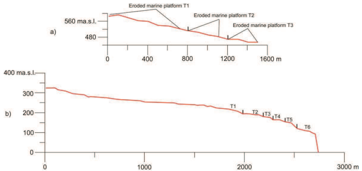
Figure 6. DGPS topographic profiles P1 (a) and P2 (b), indicated in figure 5. Vertical black bars depict the identified shoreline angles (knick points).
