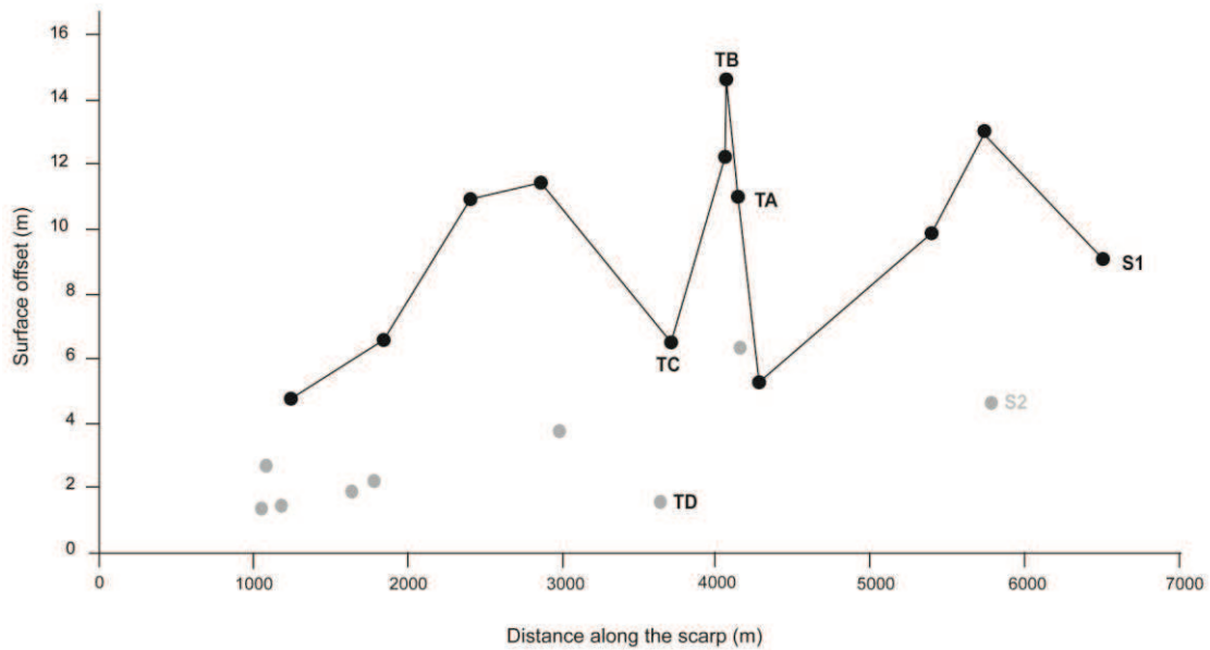
Figure 7. Shows the surface offset at both sites, where surfaces S1 (black line) and S2 (gray dots) are preserved in the footwall block. Where Surface S1 is preserved, surface offset varies between 4.7-14.7 m, and where Surface S2 is preserved surface offset varies between 1.3 and 6.3 m.
