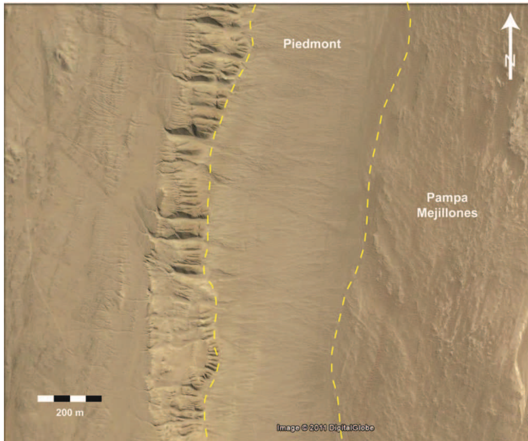
Figure 6. Google Earth image showing a portion of the southern segment of the Mejillones Fault. At this site the piedmont is constructed by a unique alluvial surface and there is no scarp present. Yellow segmented lines limit the extent of the piedmont.
