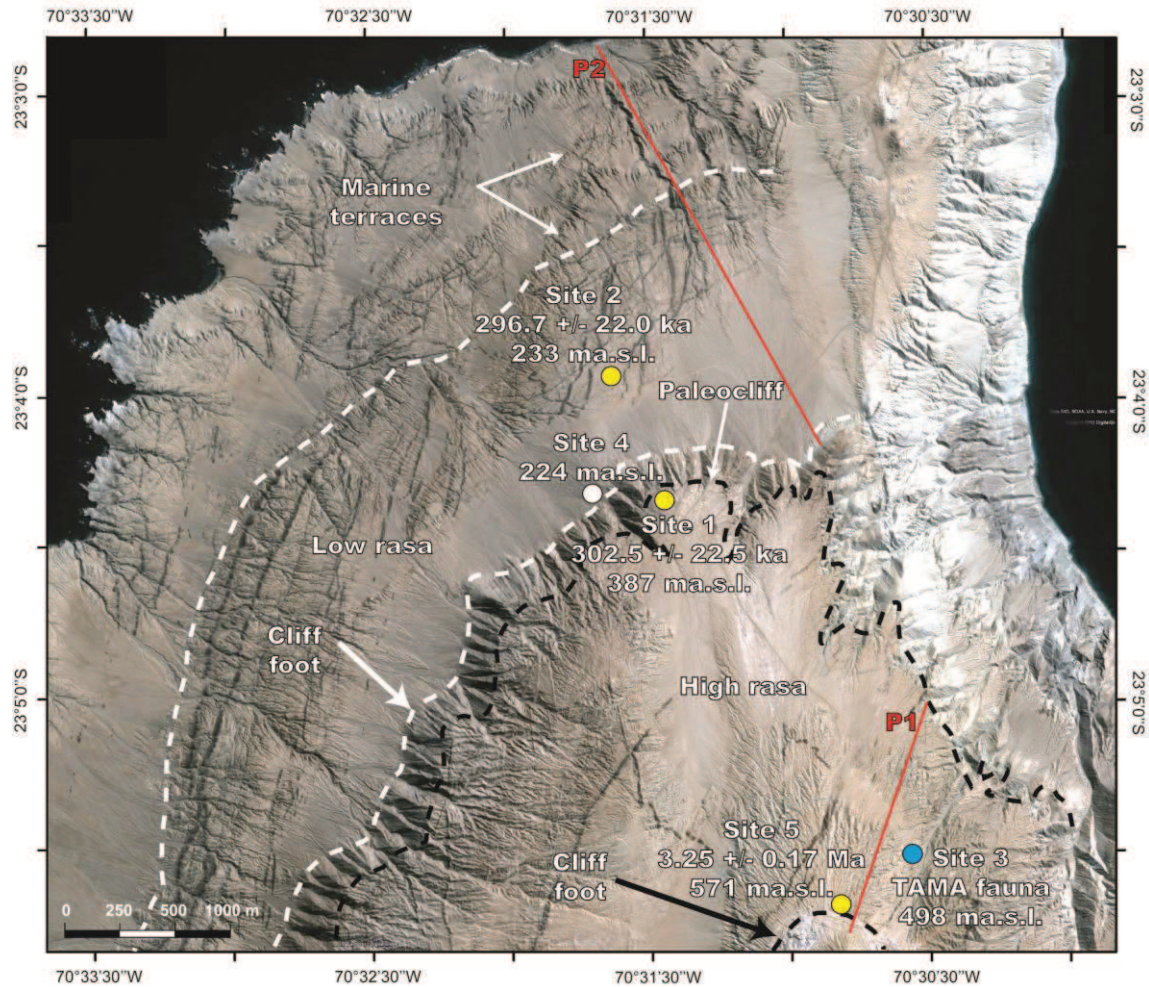
Figure 5. Google earth image showing the two rasas at the northern Morro Mejillones Horst. Black and white segmented lines limit the high and low rasas , respectively. Yellow circles are sites in which numerical ages have been constrained. Blue circles are sites where age assignments have been made. The white circle marks the elevation one of the points of the cliff-foot of the low rasa .
