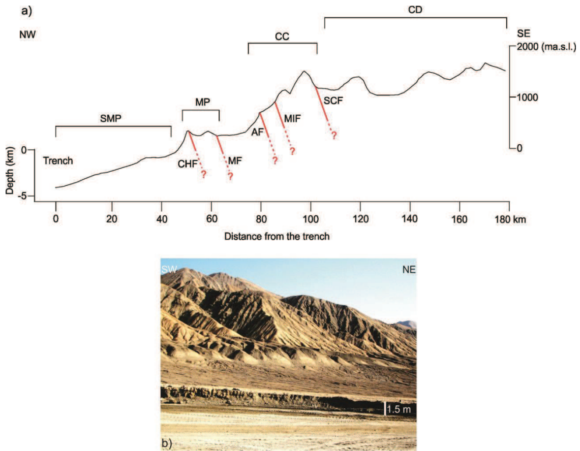
Figure 2. a) NW-SE profile made from GTOPO 90 topographic and bathymetric data. It shows the location of normal faults at \sim 23.25^{\circ}\text{S} . The represented morphotectonic domains identified in the profile are as follows: SMP= Submerged marine platform; MP= Mejillones Peninsula; CC= Coastal Cordillera; CD= Central Depression. Faults along the profile are depicted by red lines. Their prolongations in depth are represented by red segmented lines, since the root of these structures has not been precisely constrained. Interrogation signs are also put at the bottom of each prolonged fault to represent this situation. CHF= Caleta Herradura Fault; MF= Mejillones Fault; AF= Aeropuerto Fault; MIF= Mititus Fault and SCF= Salar del Carmen Fault; b) General view of the Mejillones Fault scarp.
